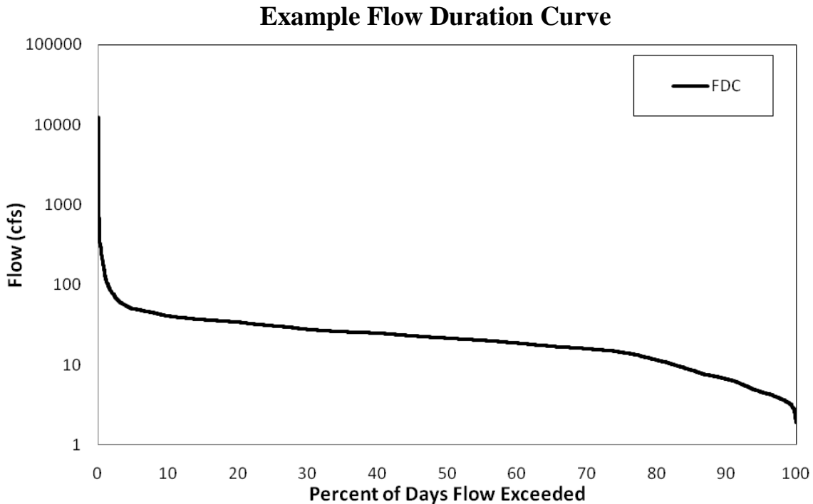
Figure 4.4. Example flow duration curve. Historical stream flow data are used to determine how frequently stream conditions exceed different flows.
